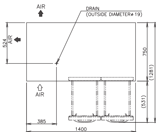
VIEW A (1/10)
