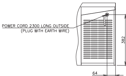
VIEW A (1/10)
